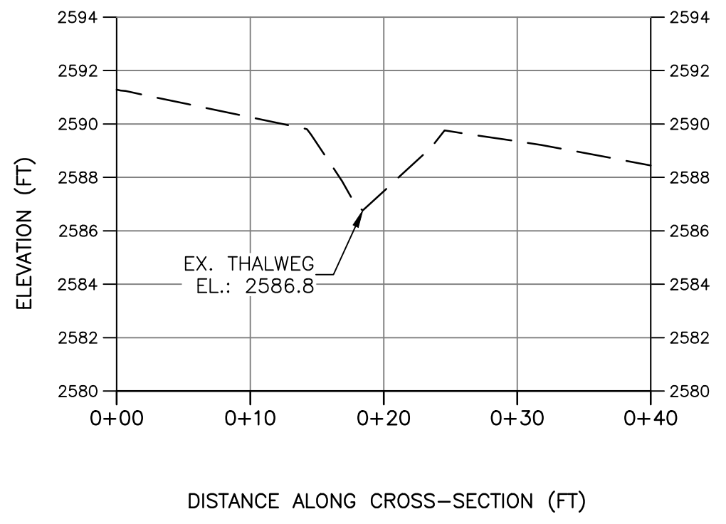
S-N10 BASELINE CROSS-SECTION A PIPE CL
