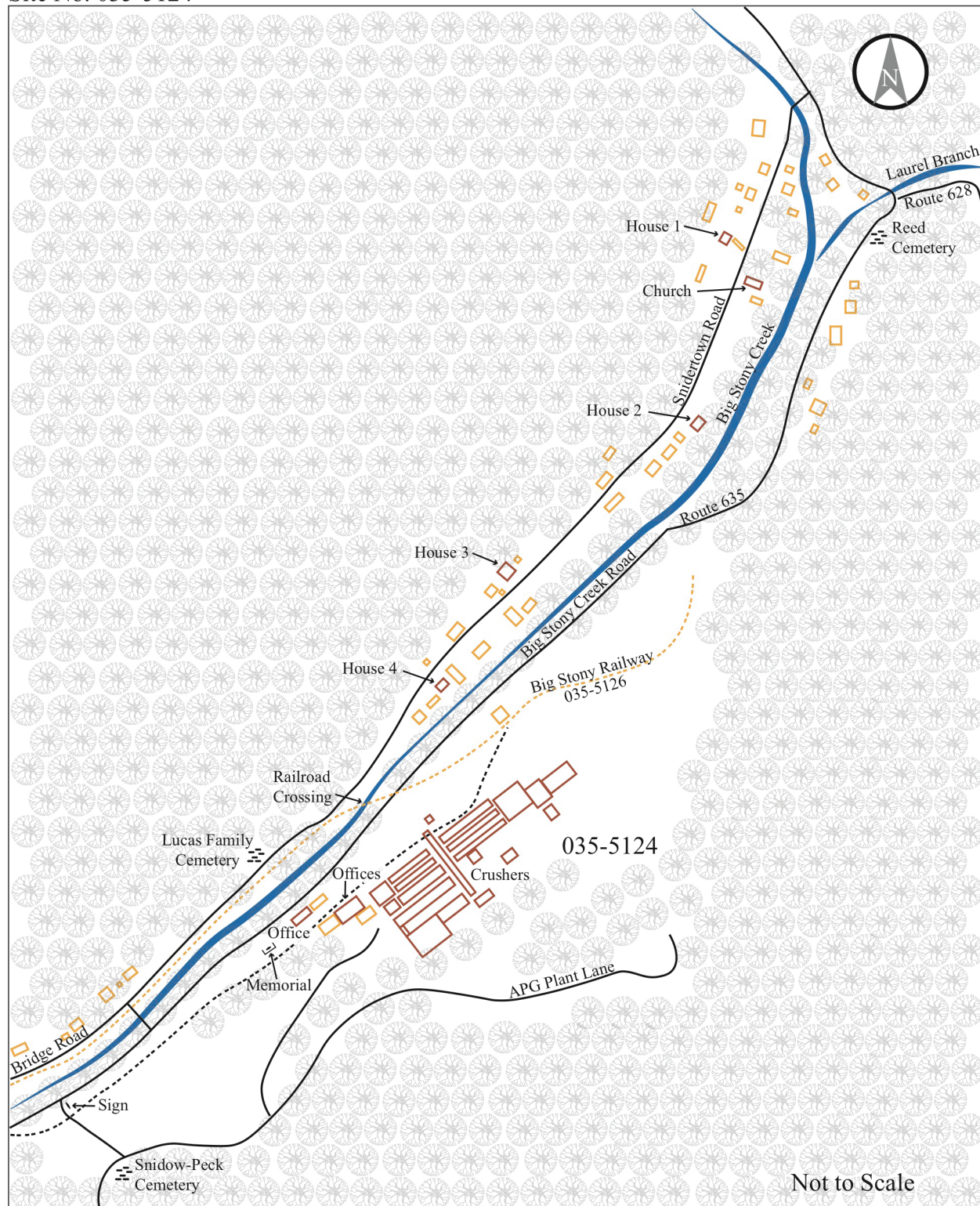
Site Map of APG Lime Corp Plant #1 (035-5124)
